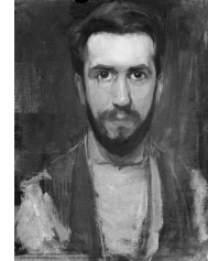
100 singular vectors
