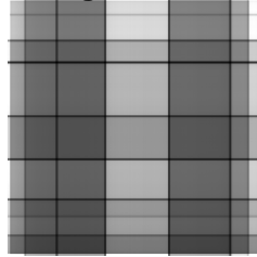
9 singular vectors
