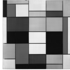
18 singular vectors
