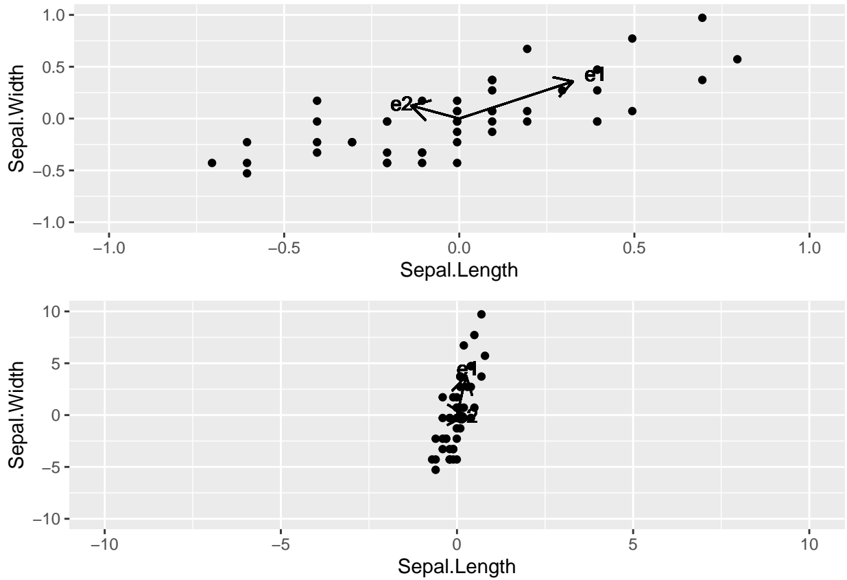
Top: original matrix – Bottom: second column of \mathbf{X} multiplied by 10 (e.g. moving from cm to mm). Directions of maximal variability are affected by the units of the variables.
