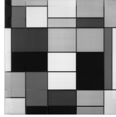
18 singular vectors
