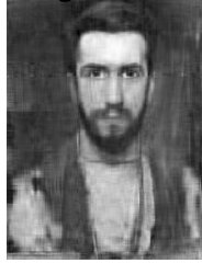
50 singular vectors
