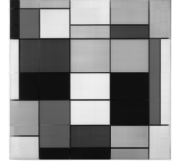
21 singular vectors
