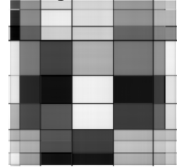
12 singular vectors
