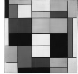
21 singular vectors
